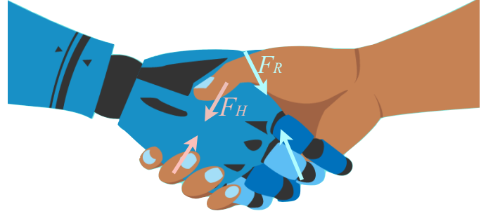
Fig. 1. Human-robot handshaking. While handshaking, human applies on the robot palm a force F_H that is measured by a set of pressure sensors, while robot applies a force F_R to human palm. In this paper we analyze some possible controllers relating F_H and F_R .
