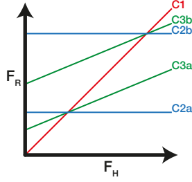
Fig. 5. F_R as a function of F_H in the proposed controllers. C1: robot follower, F_R = F_H . C2: robot open loop, F_R and F_H are independent; two levels of force are implemented: C2a (lower) and C2b (higher). C3: combined controller F_R is dependent both on F_H (as in C1) and on the robot's intrinsically preferred force (as in C2). C3a has a lower intrinsically preferred force, and C3b has a higher value.
