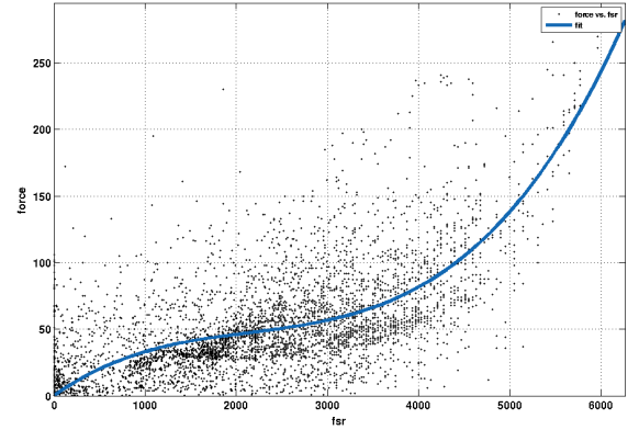
Fig. 3. Plot of F_{fsr} against F_H (measured with load cell), along with best-fit cubic polynomial.
