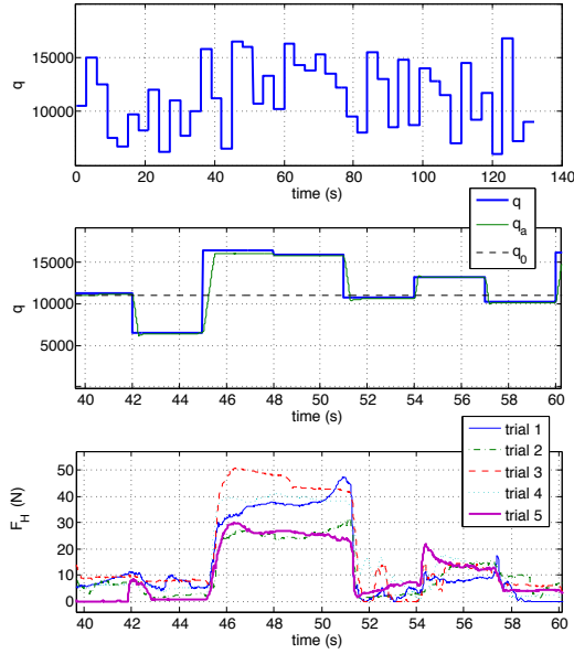
Fig. 4. Open loop test. Top: reference q profile applied in all the tests. Middle: q , q_a , q_0 profiles in a part of the experiment. Bottom: estimated F_H values for 5 different trials of the same subject, in the same experiment part.
