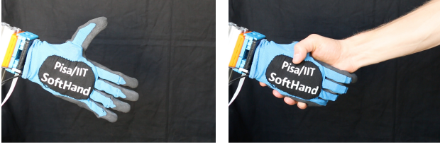
Fig. 6. Experimental setup for user study, with the robot hand attached to a fixed mount.
