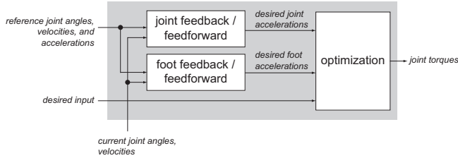
Fig. 5. Overview of the tracking controller.
