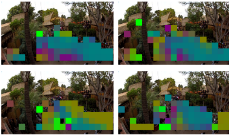
Fig. 10: Data segments of optical flows in image grids. Color coding also indicates different orientations, but in the image space.
