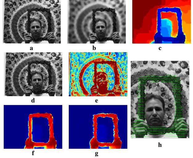
Figure 7. Real dataset (Frame): (a,d) the reference view at time t and t+1 , respectively; (b) the slice from our 3D volume that corresponds to foreground object; (c) the computed confidence map of (b), with high confidence points colored in red; (e) the estimated depth map. (f) the magnitude of the optical flow estimated by our method; (g) the magnitude of the optical flow estimated by [28]. (h) the flow map of our optical flow.
