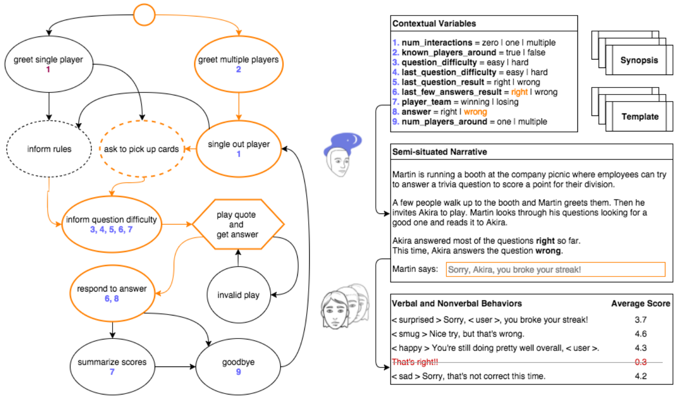
Figure 3: PIP’s goal state graph for the trivia game (left) including the number for the contextual variables used to generate narratives in the table at the top-right. Dashed lines represent conversational goals with language that was not authored by the crowd (some error handling nodes omitted for clarity). The right side contains an example of a semi-situated narrative generated by traversing the colored path through the graph to the node respond to answer . Below the narrative, some of the language behaviors produced at the end of the pipeline for that story. The line “That’s right” was rejected in the editing phase; all the other lines were added to PIP’s behavioral repertoire.
