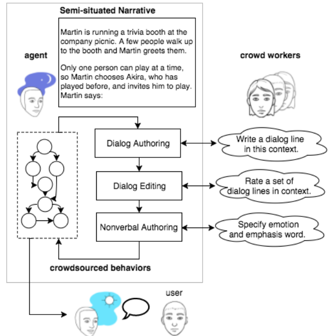
Figure 1: Overview of our semi-situated learning pipeline.
