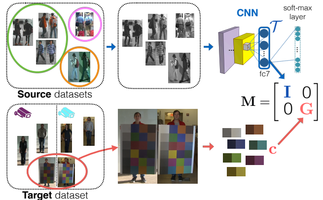
Figure 1: One-Shot Metric Learning. We split metric M into texture and color components. Deep texture features T are trained with CNN on intensity images to enforce color invariance without having to fine-tune. Joint learning on multiple source datasets (labeled data) increases good generalization under the Euclidean distance (identity matrix I ). We adapt for color differences specific to target camera pair (unlabelled data) using a single image of color chart and learning color metric G for patch color features c .
