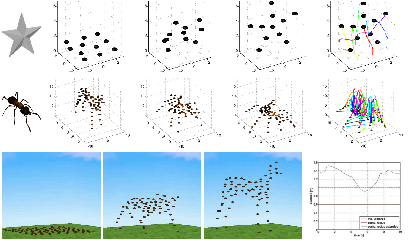
Fig. 3. Top row and left to right: Input object star; eleven simulated quad-rotor helicopters in their initial configuration, followed by an intermediate capture after 2s and in their final positions (4s) displaying the star; trajectory of each quad-rotor in different colors. Middle row and left to right: Input object ant; 80 simulated quad-rotor helicopters in their initial configuration displaying the dog, followed by an intermediate capture after 3s and in their final positions (7s) displaying the ant; trajectory of each quad-rotor in different colors. Bottom row: 80 simulated quad-rotors take off and display the dog (three screenshots at 0s, 4s and 9s; the minimum distance between quad-rotors in each time instance is shown in the right-most image. The minimum distance stays over twice the radius of the vehicles and thus collisions are avoided. Realistic background is added to visualize the effect of such a display.
