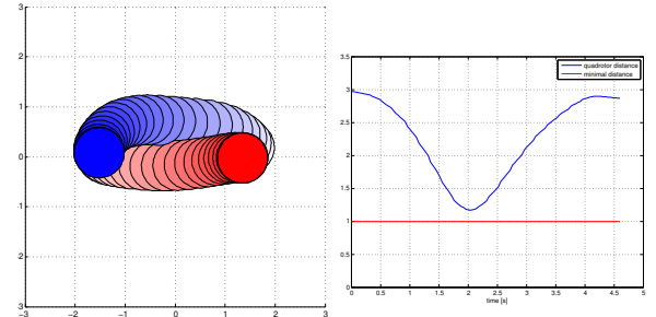
Fig. 6. Two real quadrotors exchange positions. Left: Top view of the trajectories. Right: Distance between the quadrotors at each time instance (blue) and desired minimal distance (red).
