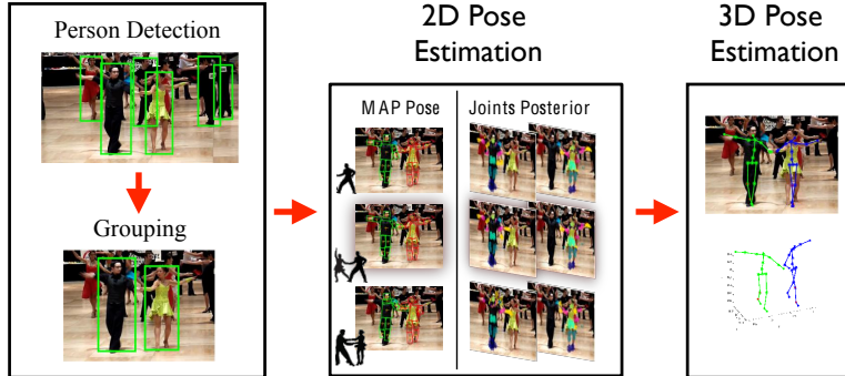
Fig. 1. Complete overview for the proposed method illustrated through an actual result obtained with our framework on a real competition dance sequence.
