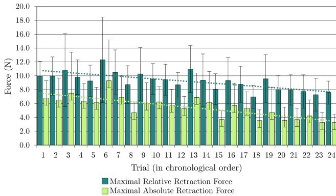
Fig. 7. Maximal forces during handover as experienced or applied by the giver over trials ordered chronologically. Lines of best fit for each are shown. Error bars represent 95% CIs.
