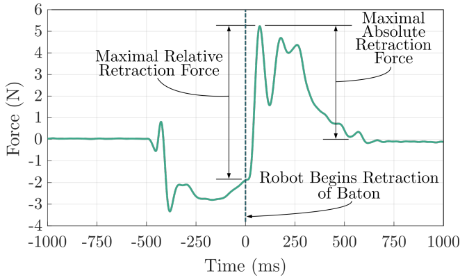
Fig. 5. Sample end effector axial force vs. time plot for a participant depicting features used in the analysis.
