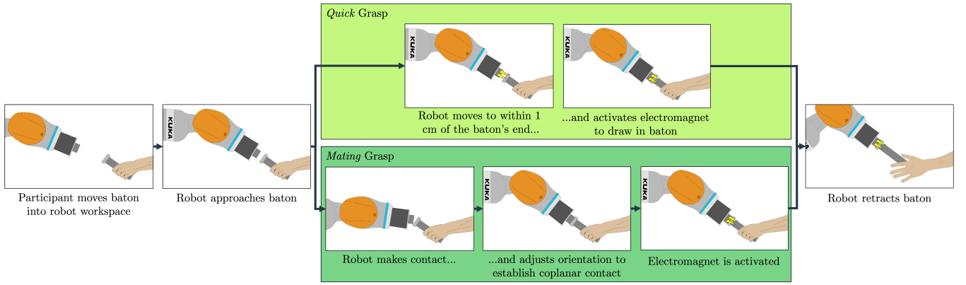
Fig. 2. Flowchart of quick (top row) and mating grasp types. The quick grasp pulls in the baton magnetically while the mating grasp establishes coplanar contact, gently pressing against the baton before activating the magnet.
