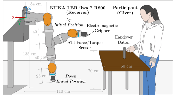
Fig. 1. Experimental setup for handover experiment. Diagram shows both the up and down initial arm positions tested as conditions in the experiment.
