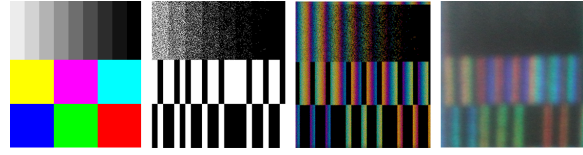
Figure 8: A 9 \times 9 pixel input image (left), the stochastically dithered mask (middle left), simulated image (middle right) and a macro photograph of a physical projection of size 8.4 \times 8.4 mm (right).
