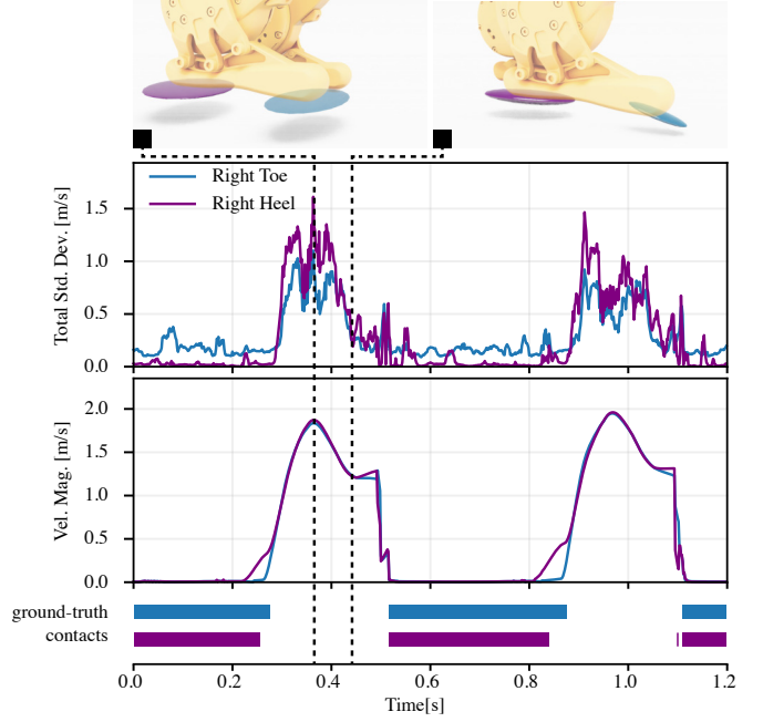
Fig. 3: Contact Covariance. Visualization of the contact covariance total standard deviation \sqrt{\text{tr}(\Sigma_{C_i}^B)} and contact point velocity magnitude during a forward-walking gait of our robot, along with ground-truth contacts.
