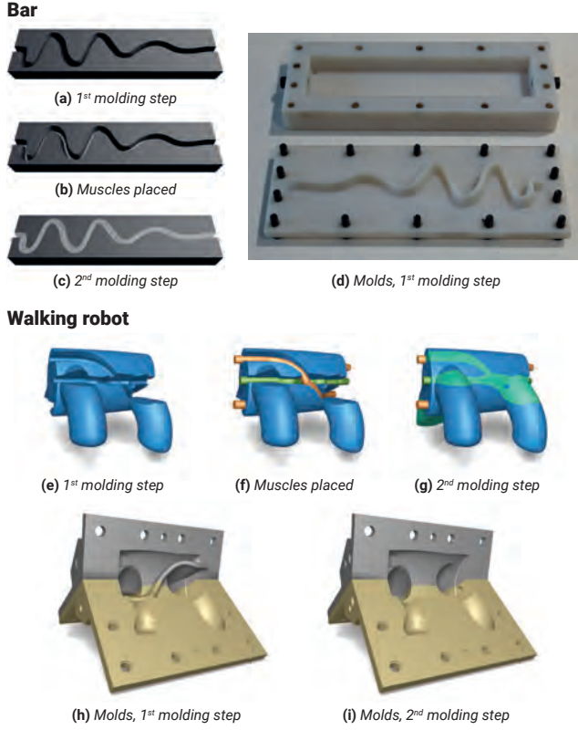
Fig. 7. Fabrication process. Steps and mold designs for Bar (Fig. 10) and Walking robot (Fig. 16). First, the robot is fabricated with grooves for the artificial muscles (a, e). The muscles are then placed in the grooves (b, f), and overmolded (c, g). Note that for (h) and (i), one mold part is not shown.
