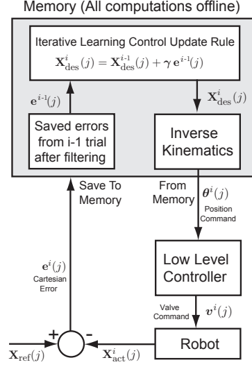
Fig. 3. Block diagram of our end-effector space iterative learning control algorithm. We filter the cartesian space errors e^{i-1}(j) using a zero phase filter before applying the iterative learning update rule. The super-script i denotes the trial number and j denotes a time instance.
